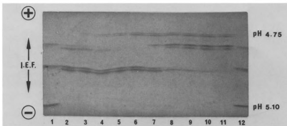
Fig.3. Here a Gc 1F-1S serum is used to demonstrate the importance of the pI differences between the proteins in their affinities for the ligand. A progressive saturation with the 25-OH- D_3 solution is obtained. In samples 1,12, the 3 bands obtained after IEF correspond to a Gc 2-1F serum. The most cathodic band corresponds to the Gc 2 protein. In the anodic zone the set of 2 bands corresponds to the Gc 1F protein. In sample 2 the electrophoretic pattern obtained corresponds to Gc 1F-1S serum. Four bands are observed. The Gc 1Sc and Gc 1Fc protein bands are the more cathodic bands while the Gc 1Fa and Gc 1Sa protein bands are the more anodic bands; samples 3-11 show the results of the progressive addition of 25-OH- D_3 (0.25, 0.33, 0.5, 0.7, 1, 1.4, 1.8, 2 and 3 \mu g 25-OH- D_3 /ml serum, respectively) to the Gc 1F-1S sample.
