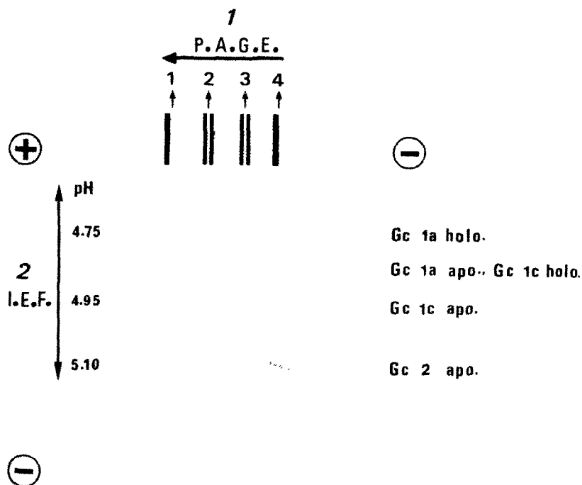
Fig.1. Two-dimensional electrophoretic pattern of a Gc 2-1 sample partially saturated with 25-OH-D 3 (1 \mu g/ml serum). The band positions after the first dimension (PAGE) are: (arrow 1) Gc 1a holoprotein; (arrow 2) Gc 1a apoprotein, Gc 1c holoprotein; (arrow 3) Gc 1c apoprotein, Gc 2 holoprotein; (arrow 4) Gc 2 apoprotein. Each holoprotein form presents an anodic mobility while the excess of the protein bands in the apoprotein form shows a cathodic mobility. During the second dimension (IEF) the protein-ligand exchange takes place to the detriment of the Gc 2 holoprotein.
